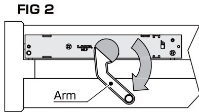
FIG 2-3 : ① Pull the arm out and close the door slowly until the arm touches the door. ② Insert the template between the arm and the door so that the arm roller fits in the square hole shown on the template. ③ Adjust the template so that it is parallel with the top of the door and mark the screw hole shown on the template.
