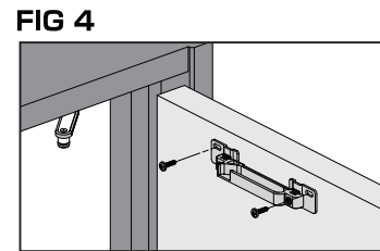
FIG 4 : Fix the strike plate with the installation screws provided.
