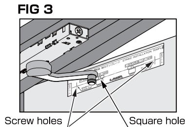
FIG 2-3 : ① Pull the arm out and close the door slowly until the arm touches the door. ② Insert the template between the arm and the door so that the arm roller fits in the square hole shown on the template. ③ Adjust the template so that it is parallel with the top of the door and mark the screw hole shown on the template.
